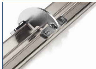
Rack stop trolley stops for rails that are screwed into position
